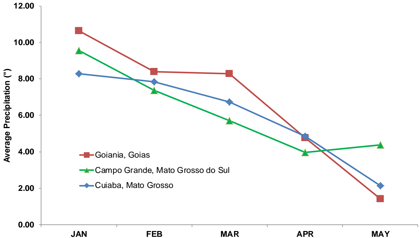
Average Precipitation In Center-West Brazil (") 1960 - 1990
